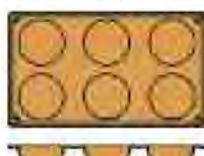
FR001 impronte cad. 6 / moulds each Ø 70 mm h 35 mm - Ø 2,75 in. h 1,37 in.
