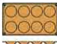
FR040 impronte cad. 8 / moulds each Ø 60 mm h 17 mm - Ø 2,36 in. h 0,66 in.
